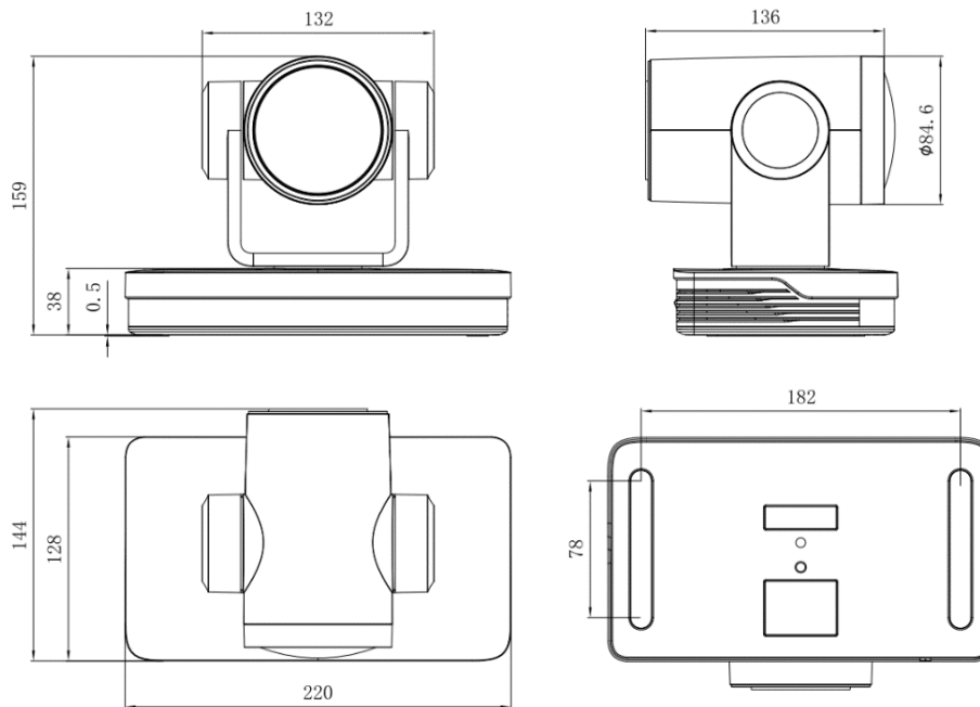
Figure2-1 Product Dimension
